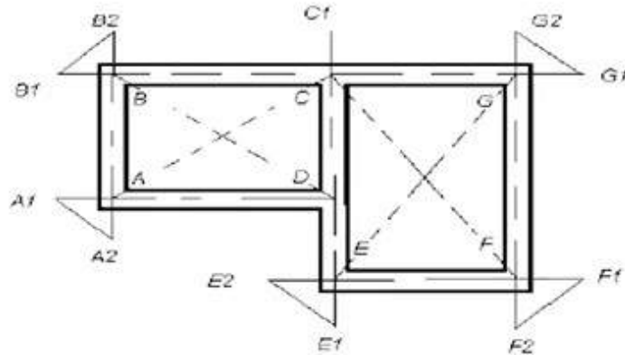
Fig.1: Example plan to be set out on the ground
